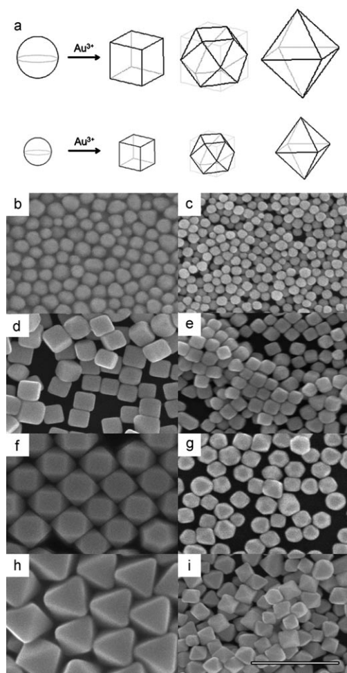
Figure 3. a) Size and shape control of gold polyhedral nanocrystals from spherical seeds. SEM images of b, c) spherical seeds (average diameters: 81 \pm 8 and 49 \pm 5 nm), d, e) cubes (average edge lengths: 116 \pm 11 and 67 \pm 6 nm), f, g) cuboctahedra ( 122 \pm 13 and 54 \pm 8 nm), and h, i) octahedra ( 236 \pm 19 and 88 \pm 10 nm). The bar represents 500 nm.
